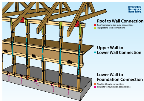
Continuous Load Path To Resist Uplift Forces
